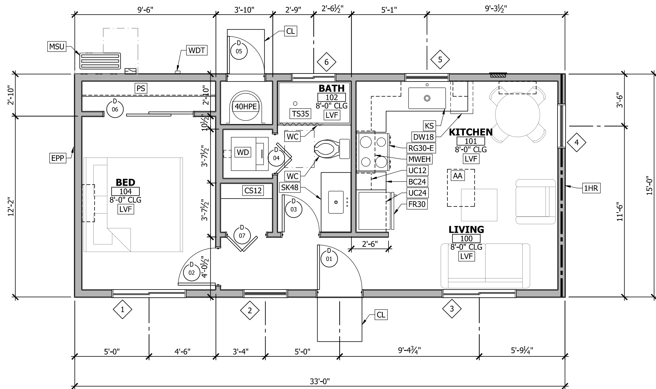
1 FLOOR PLAN A2.1 1/4" = 1'-0"
