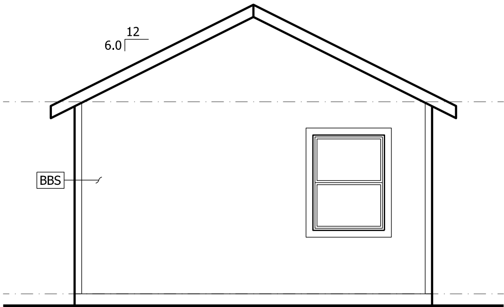
C RIGHT ELEVATION A2.1 1/4" = 1'-0"
