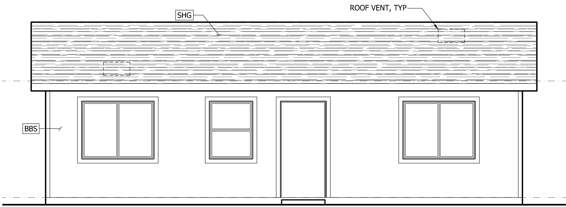
A FRONT ELEVATION A2.1 1/4" = 1'-0"
