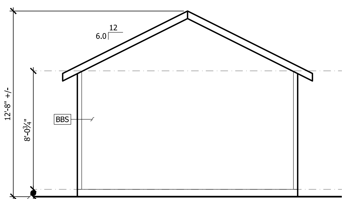
B LEFT ELEVATION A2.1 1/4" = 1'-0"
